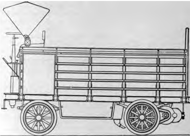
FIG. 298.—Chain and Sprocket Double Reduction for Heavy Trucks. As here shown, the motor is hung above the springs, missing the jars of travel.
